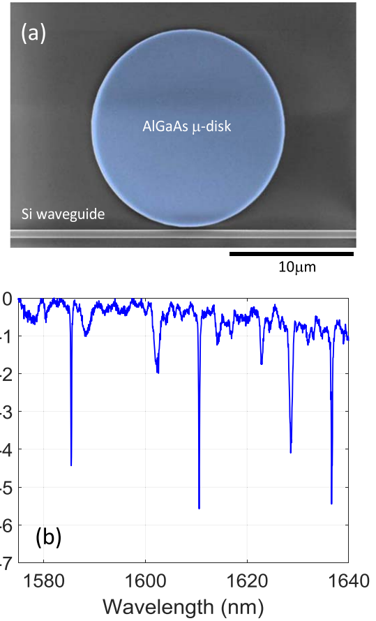
Figure 15. (a) False colour SEM image of an AlGaAs \mu -disk integrated with a silicon waveguide by direct transfer printing. (b) Measured transmission spectrum of the hybrid device.
